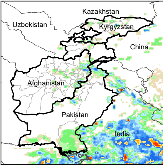
Daily Rainfall estimate for 3 Sep., 2011
