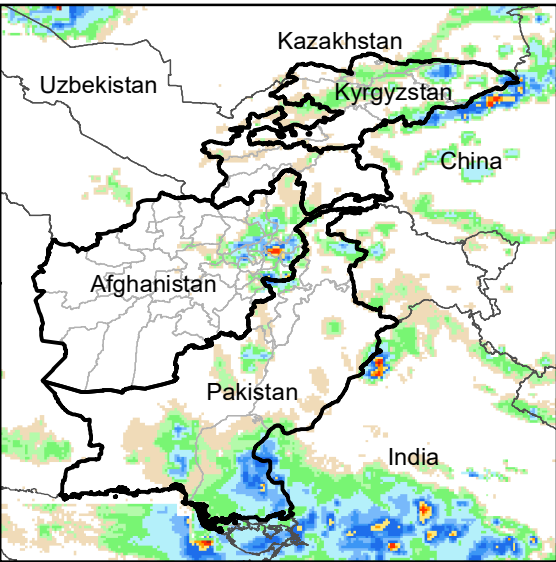
Daily Rainfall estimate for 1 Sep., 2011
