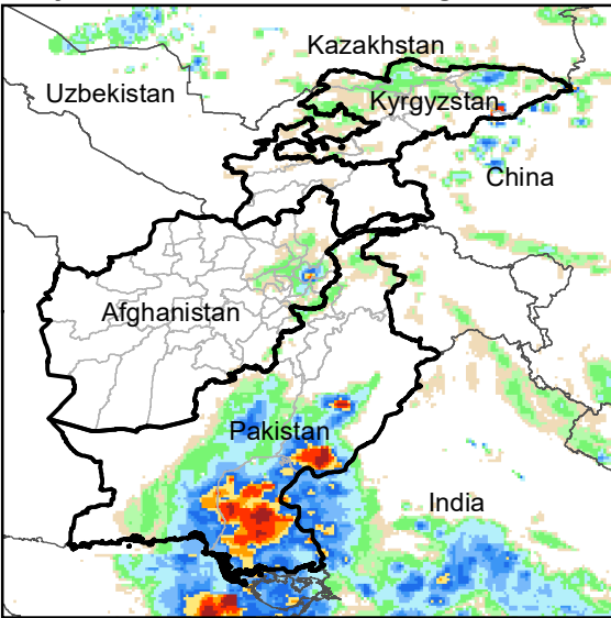
Daily Rainfall estimate for 2 Sep., 2011
