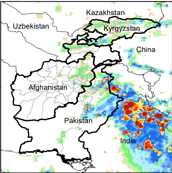
Daily Rainfall estimate for 18 Sep., 2011
