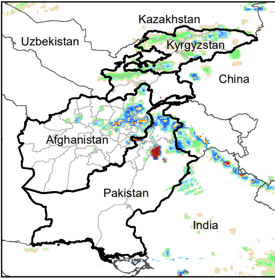
Daily Rainfall estimate for 19 Sep., 2011
