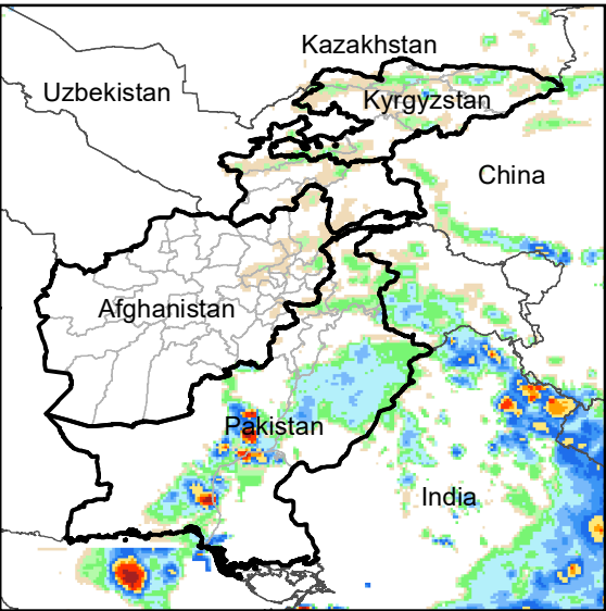
Daily Rainfall estimate for 17 Sep., 2011
