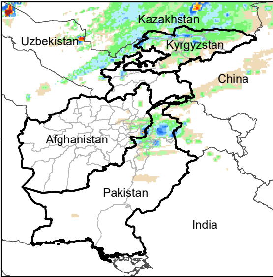
Daily Rainfall estimate for 5 Oct., 2011
