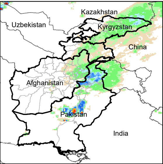
Daily Rainfall estimate for 10 Oct., 2011
