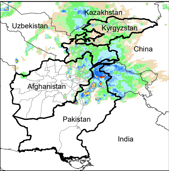
Daily Rainfall estimate for 26 Oct., 2011
