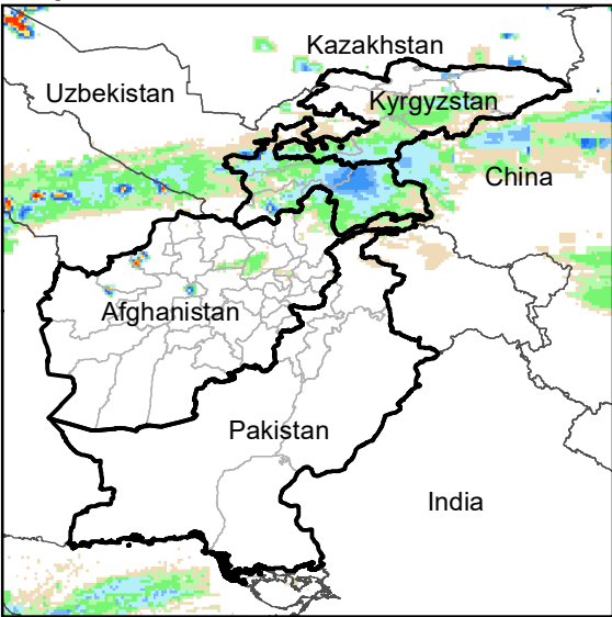
Daily Rainfall estimate for 2 Nov., 2011
