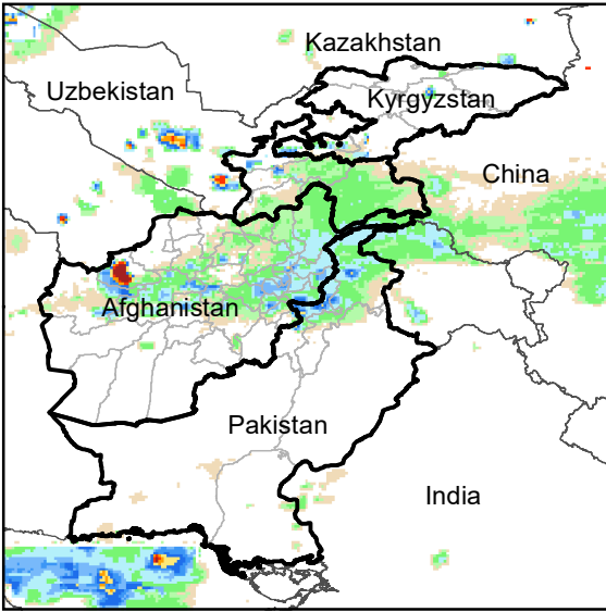
Daily Rainfall estimate for 3 Nov., 2011
