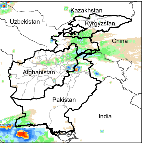
Daily Rainfall estimate for 5 Nov., 2011
