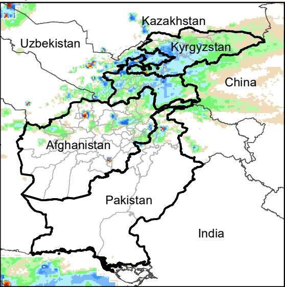
Daily Rainfall estimate for 4 Nov., 2011
