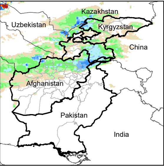
Daily Rainfall estimate for 17 Nov., 2011
