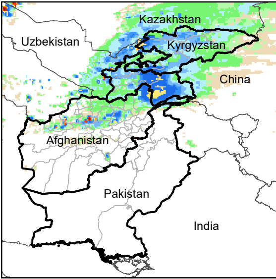
Daily Rainfall estimate for 18 Nov., 2011
