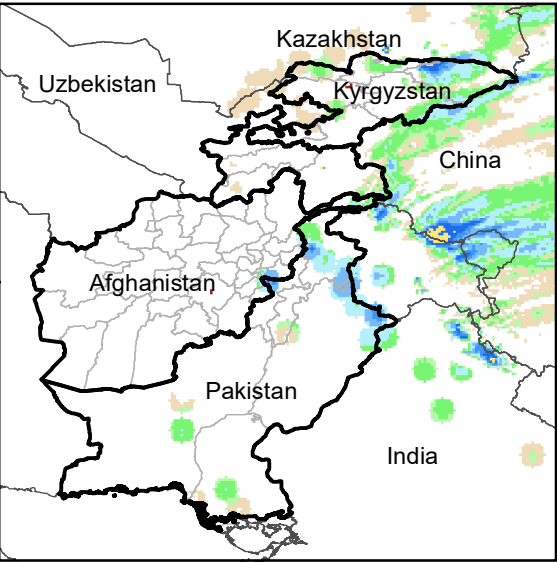
Daily Rainfall estimate for 16 Jan., 2012
