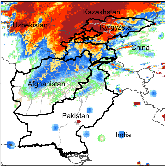
Daily Rainfall estimate for 2 Feb., 2012
