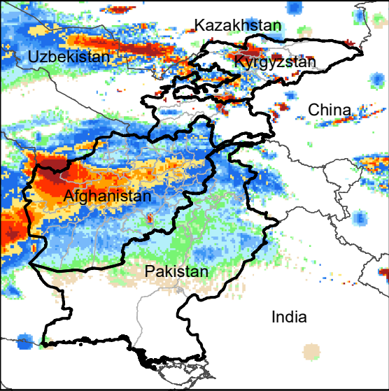
Daily Rainfall estimate for 1 Feb., 2012
