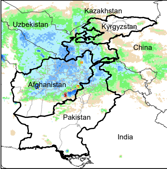
Daily Rainfall estimate for 3 Feb., 2012
