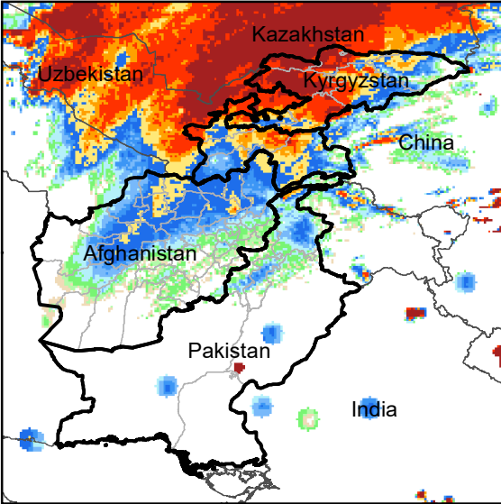
Daily Rainfall estimate for 30 Jan., 2012
