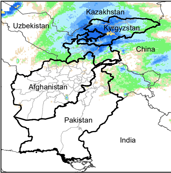
Daily Rainfall estimate for 27 Feb., 2012
