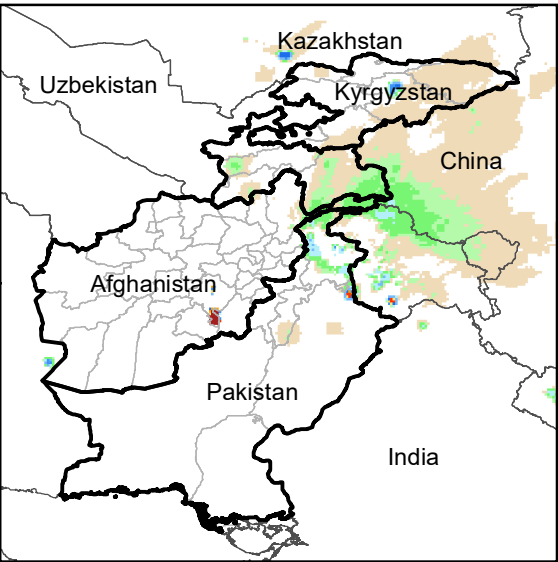
Daily Rainfall estimate for 25 Feb., 2012
