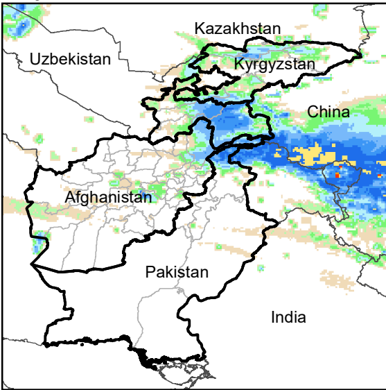
Daily Rainfall estimate for 17 Mar., 2012
