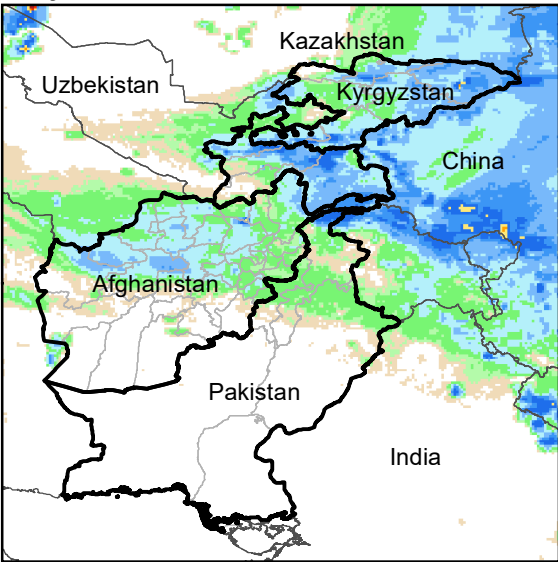
Daily Rainfall estimate for 16 Mar., 2012
