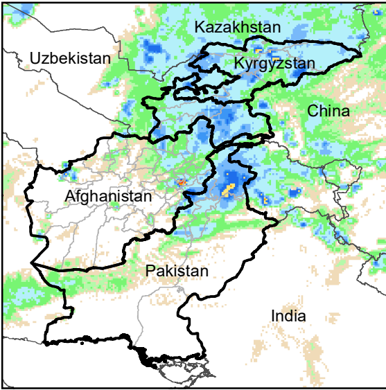
Daily Rainfall estimate for 1 Apr., 2012
