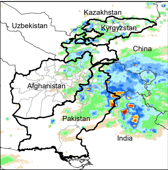
Daily Rainfall estimate for 13 Apr., 2012
