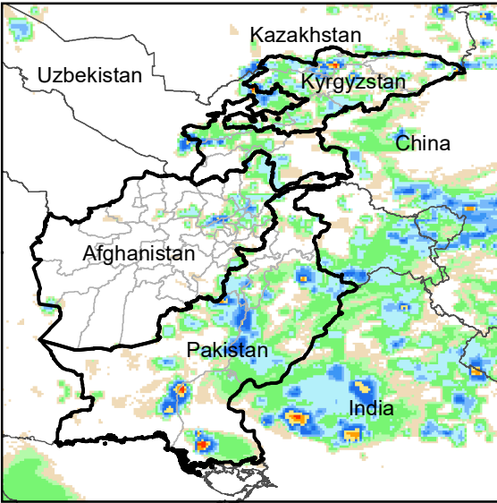
Daily Rainfall estimate for 14 Apr., 2012
