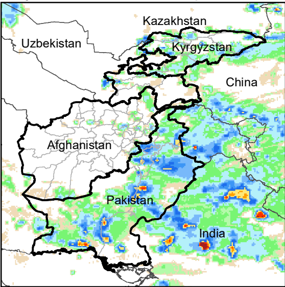
Daily Rainfall estimate for 16 Apr., 2012
