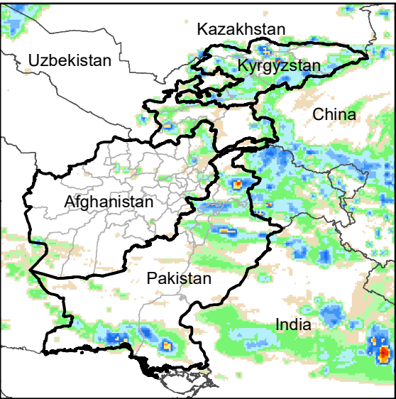
Daily Rainfall estimate for 15 Apr., 2012
