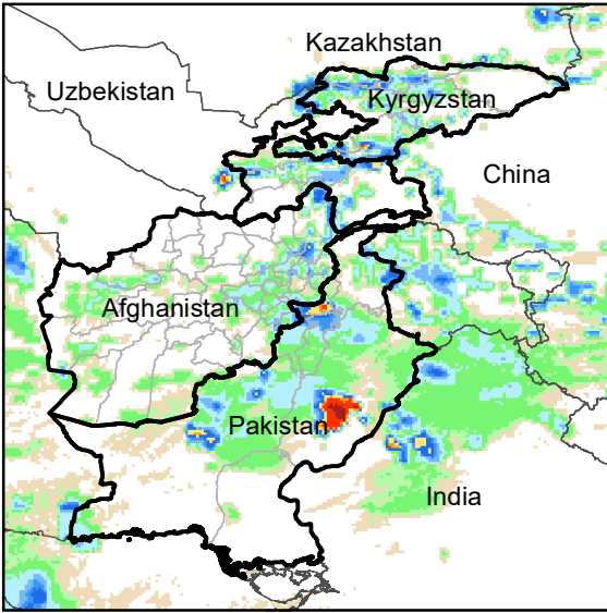
Daily Rainfall estimate for 17 Apr., 2012
