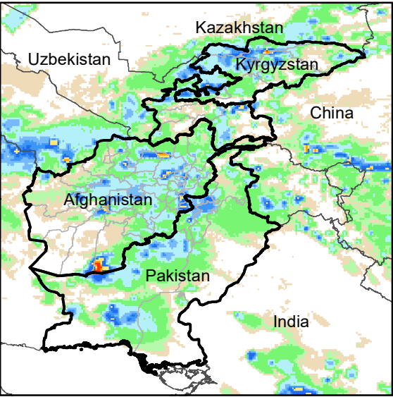
Daily Rainfall estimate for 6 May., 2012
