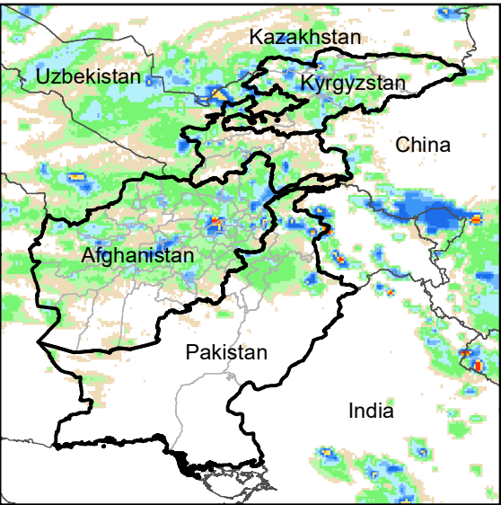
Daily Rainfall estimate for 8 May., 2012
