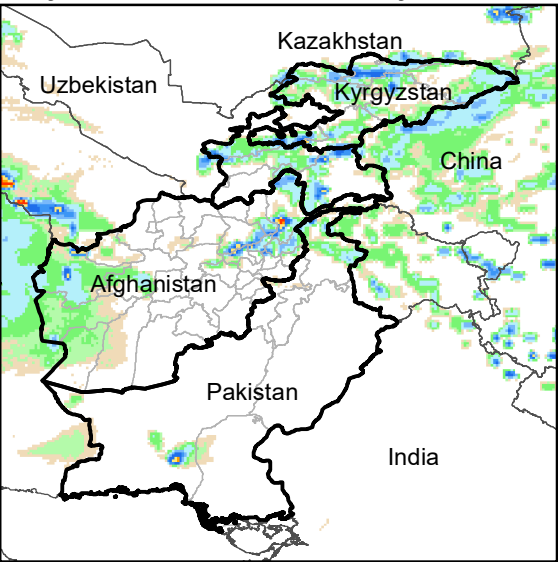
Daily Rainfall estimate for 26 May., 2012
