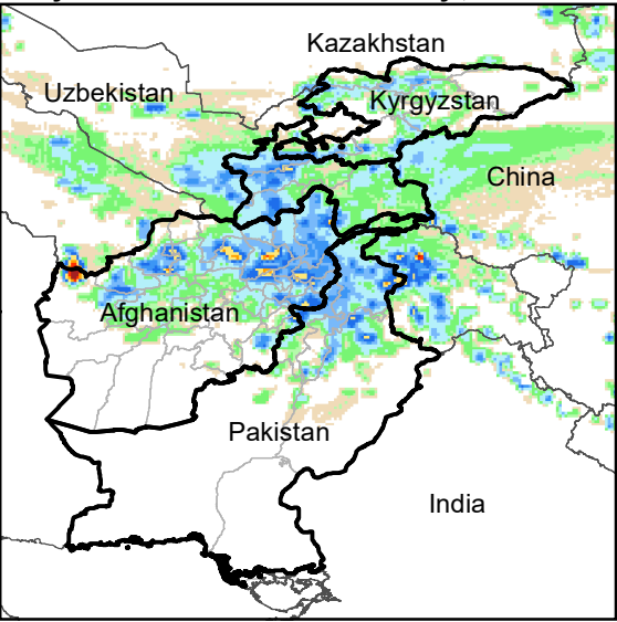
Daily Rainfall estimate for 25 May., 2012
