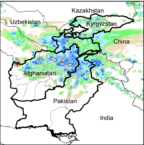
Daily Rainfall estimate for 28 May., 2012
