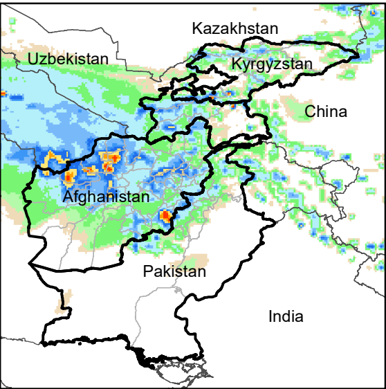
Daily Rainfall estimate for 27 May., 2012
