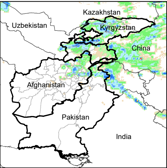
Daily Rainfall estimate for 3 Jun., 2012
