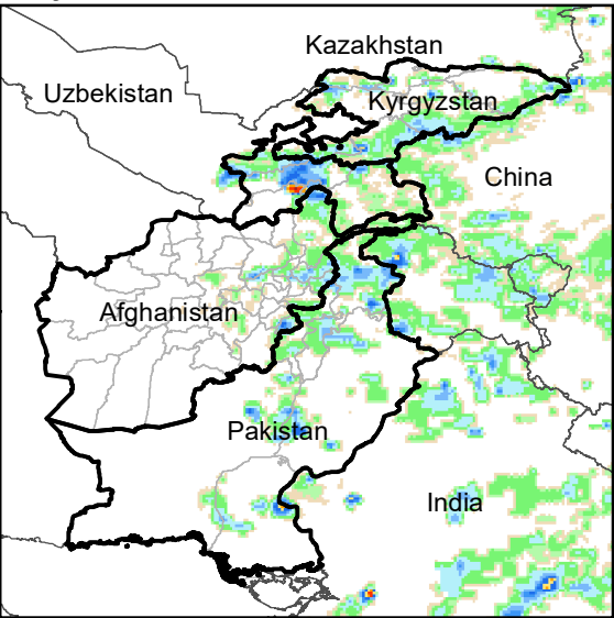
Daily Rainfall estimate for 10 Jun., 2012
