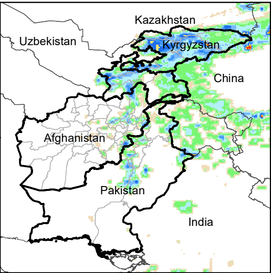
Daily Rainfall estimate for 11 Jun., 2012
