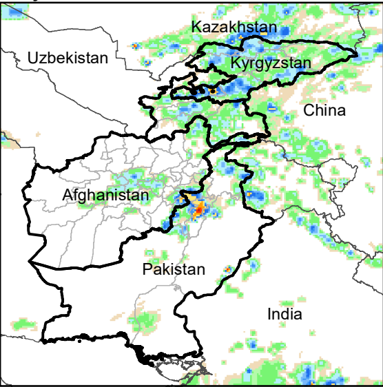
Daily Rainfall estimate for 12 Jun., 2012
