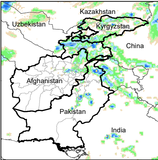
Daily Rainfall estimate for 14 Jun., 2012
