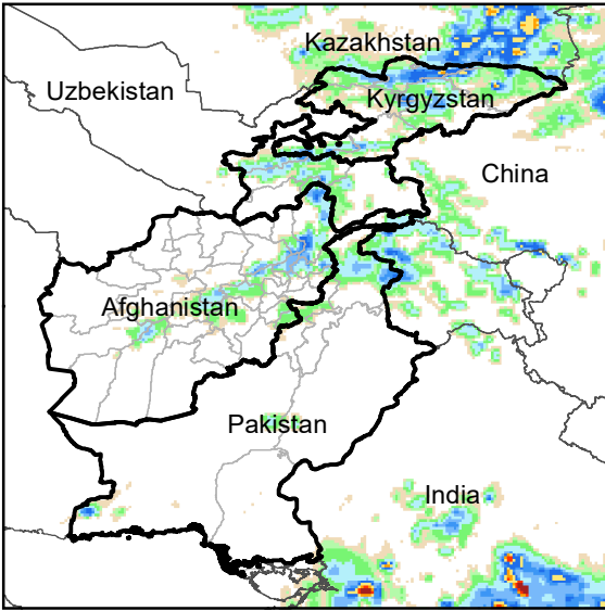
Daily Rainfall estimate for 16 Jun., 2012
