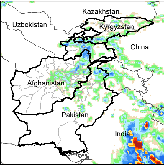
Daily Rainfall estimate for 18 Jun., 2012
