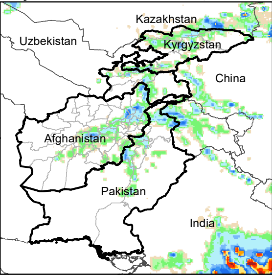
Daily Rainfall estimate for 17 Jun., 2012
