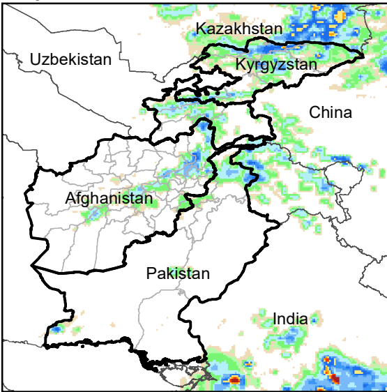
Daily Rainfall estimate for 19 Jun., 2012
