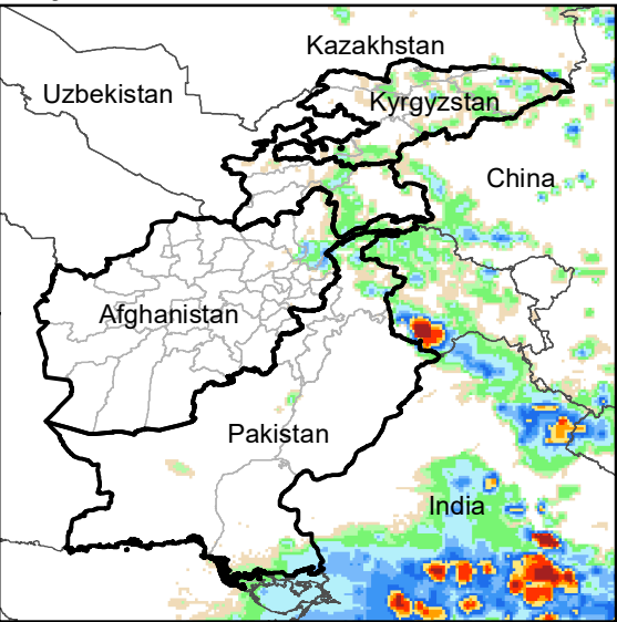
Daily Rainfall estimate for 7 Jul., 2012
