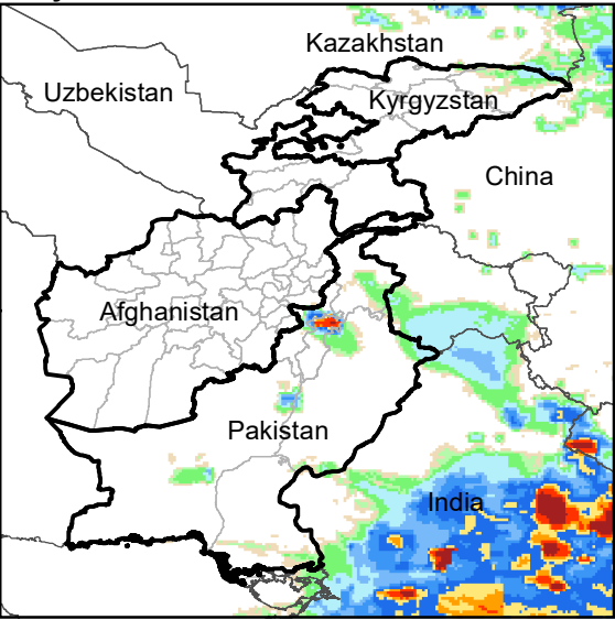
Daily Rainfall estimate for 5 Jul., 2012
