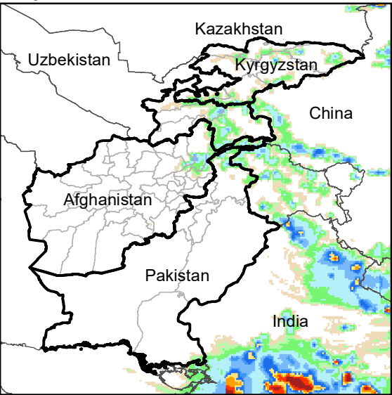
Daily Rainfall estimate for 6 Jul., 2012
