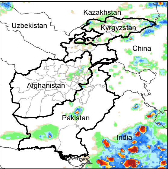
Daily Rainfall estimate for 12 Jul., 2012
