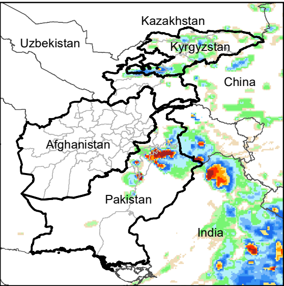
Daily Rainfall estimate for 10 Jul., 2012
