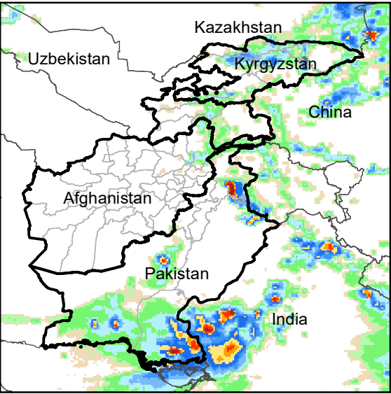
Daily Rainfall estimate for 11 Jul., 2012
