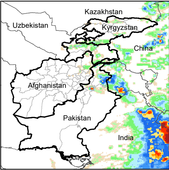
Daily Rainfall estimate for 3 Aug., 2012
