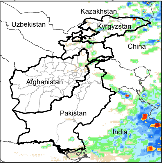
Daily Rainfall estimate for 2 Aug., 2012
