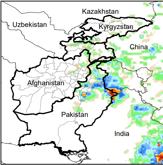
Daily Rainfall estimate for 4 Aug., 2012
