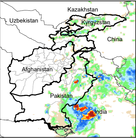
Daily Rainfall estimate for 14 Aug., 2012
