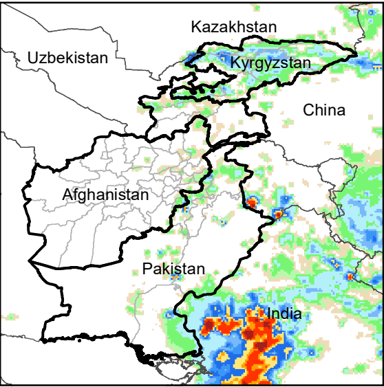
Daily Rainfall estimate for 13 Aug., 2012
