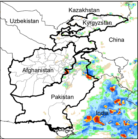
Daily Rainfall estimate for 12 Aug., 2012
