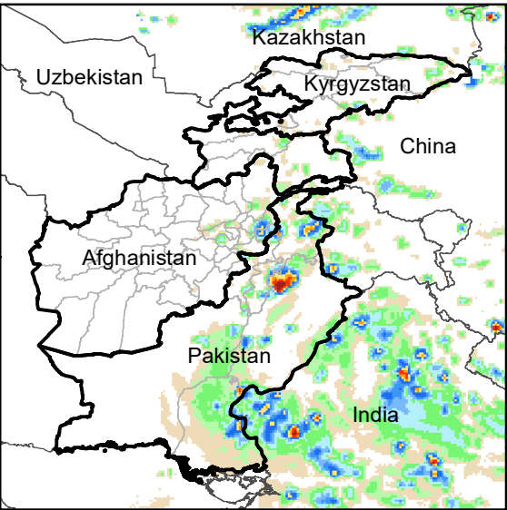
Daily Rainfall estimate for 31 Aug., 2012
