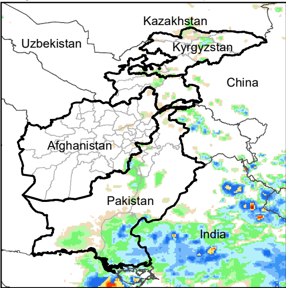
Daily Rainfall estimate for 15 Sep., 2012
