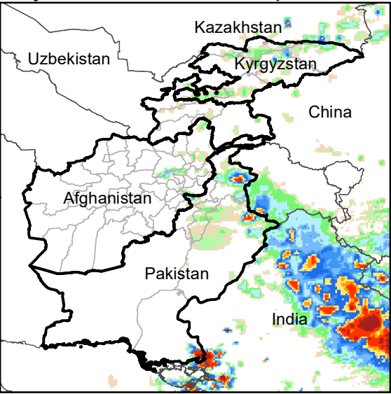
Daily Rainfall estimate for 14 Sep., 2012
