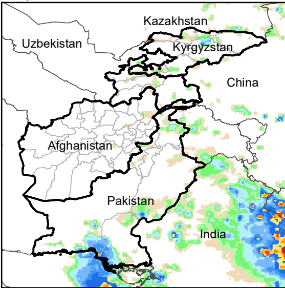
Daily Rainfall estimate for 16 Sep., 2012
