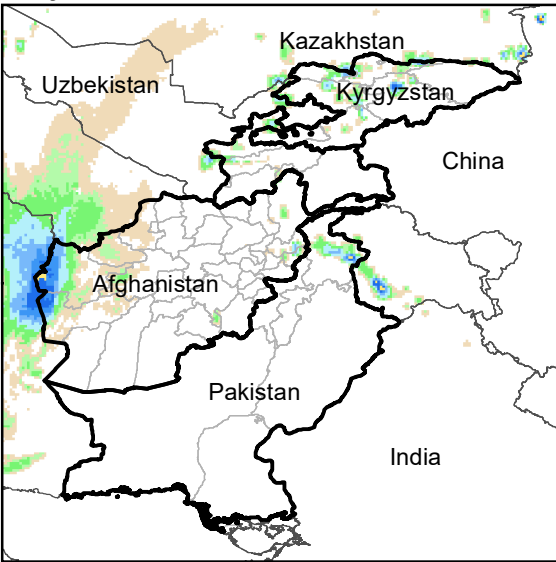
Daily Rainfall estimate for 2 Nov., 2012
