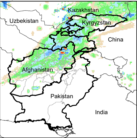
Daily Rainfall estimate for 19 Nov., 2012
