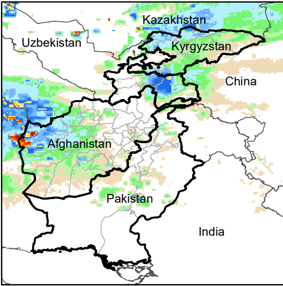
Daily Rainfall estimate for 12 Dec., 2012
