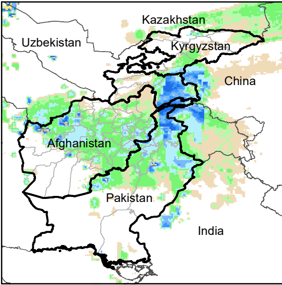
Daily Rainfall estimate for 13 Dec., 2012
