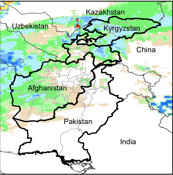
Daily Rainfall estimate for 26 Dec., 2012
