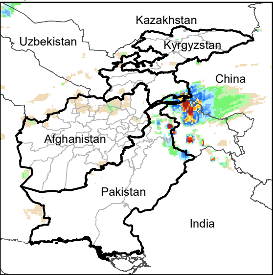
Daily Rainfall estimate for 1 Jan., 2013
