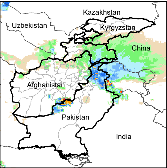
Daily Rainfall estimate for 31 Dec., 2012
