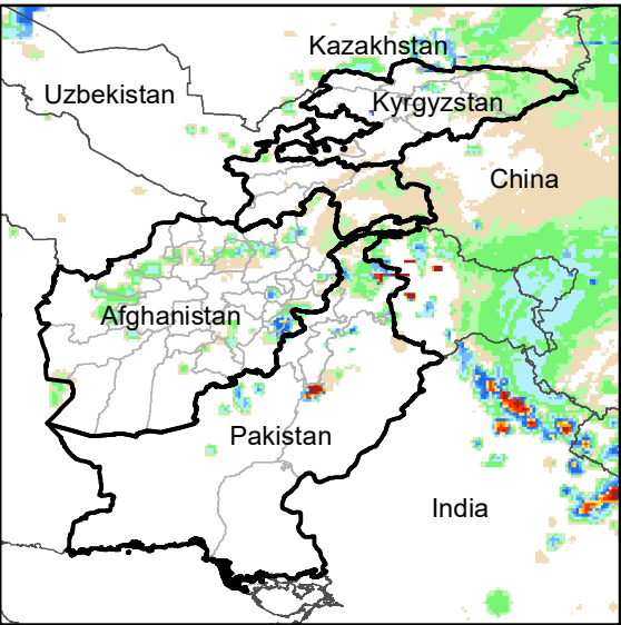
Daily Rainfall estimate for 9 Feb., 2013
