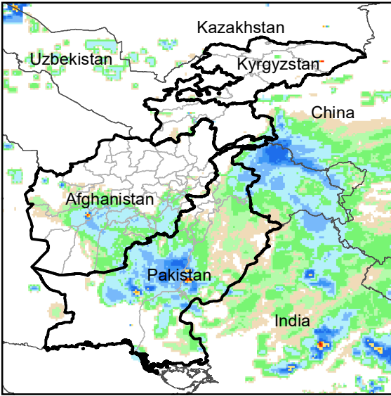
Daily Rainfall estimate for 15 Feb., 2013
