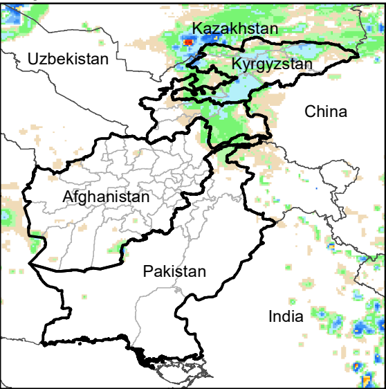
Daily Rainfall estimate for 27 Feb., 2013
