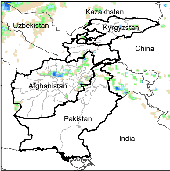
Daily Rainfall estimate for 5 Mar., 2013
