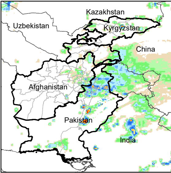
Daily Rainfall estimate for 3 Apr., 2013
