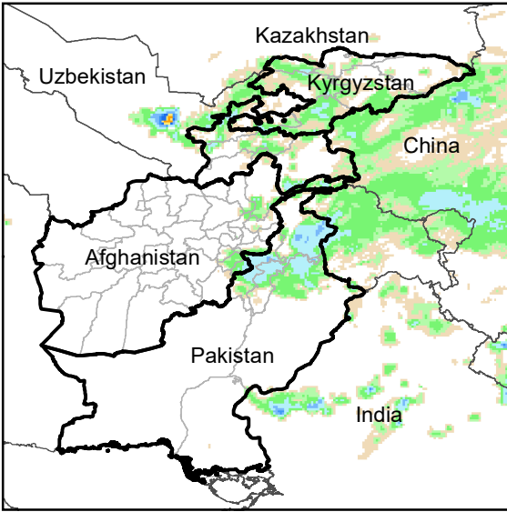
Daily Rainfall estimate for 12 May., 2013
