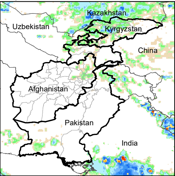
Daily Rainfall estimate for 8 Jun., 2013
