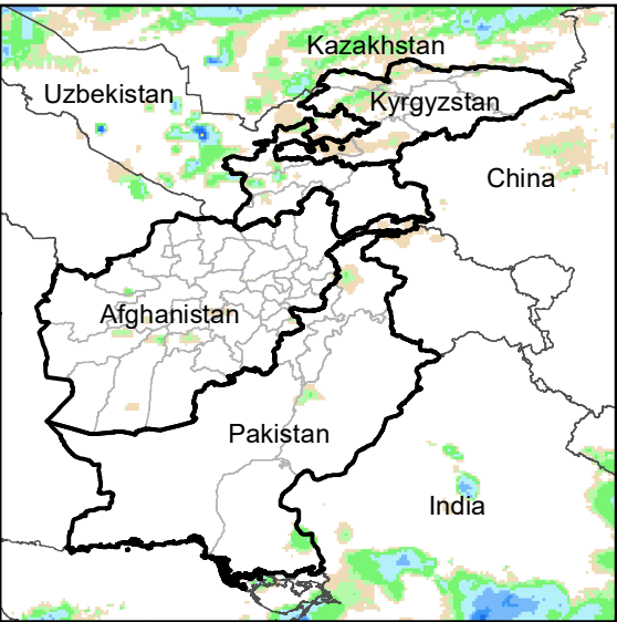
Daily Rainfall estimate for 7 Jun., 2013
