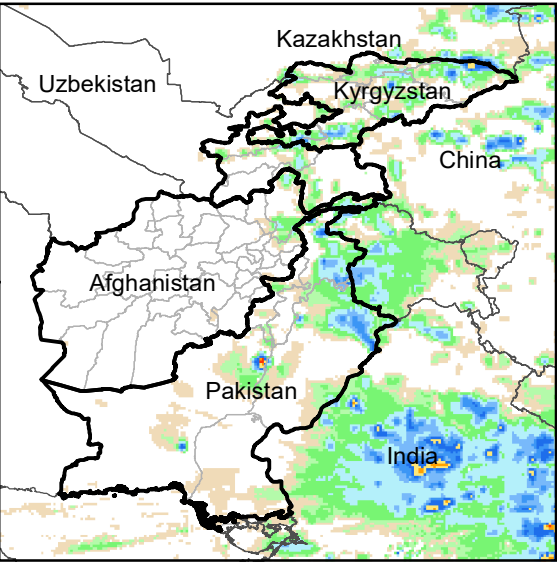
Daily Rainfall estimate for 7 Jul., 2013
