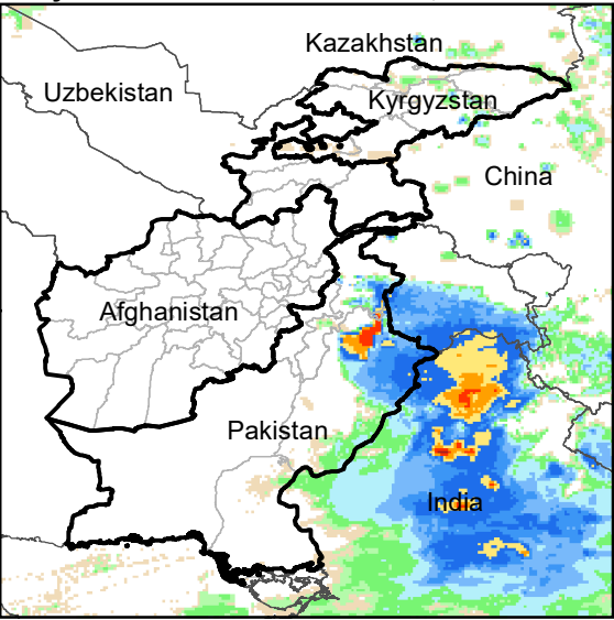
Daily Rainfall estimate for 8 Jul., 2013
