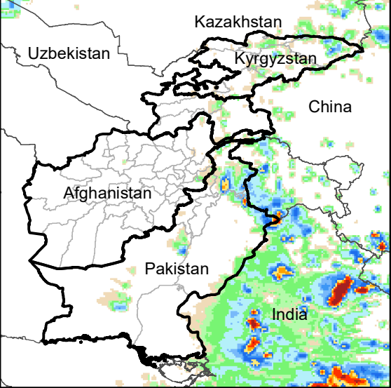
Daily Rainfall estimate for 17 Jul., 2013
