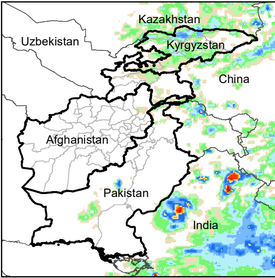
Daily Rainfall estimate for 21 Jul., 2013
